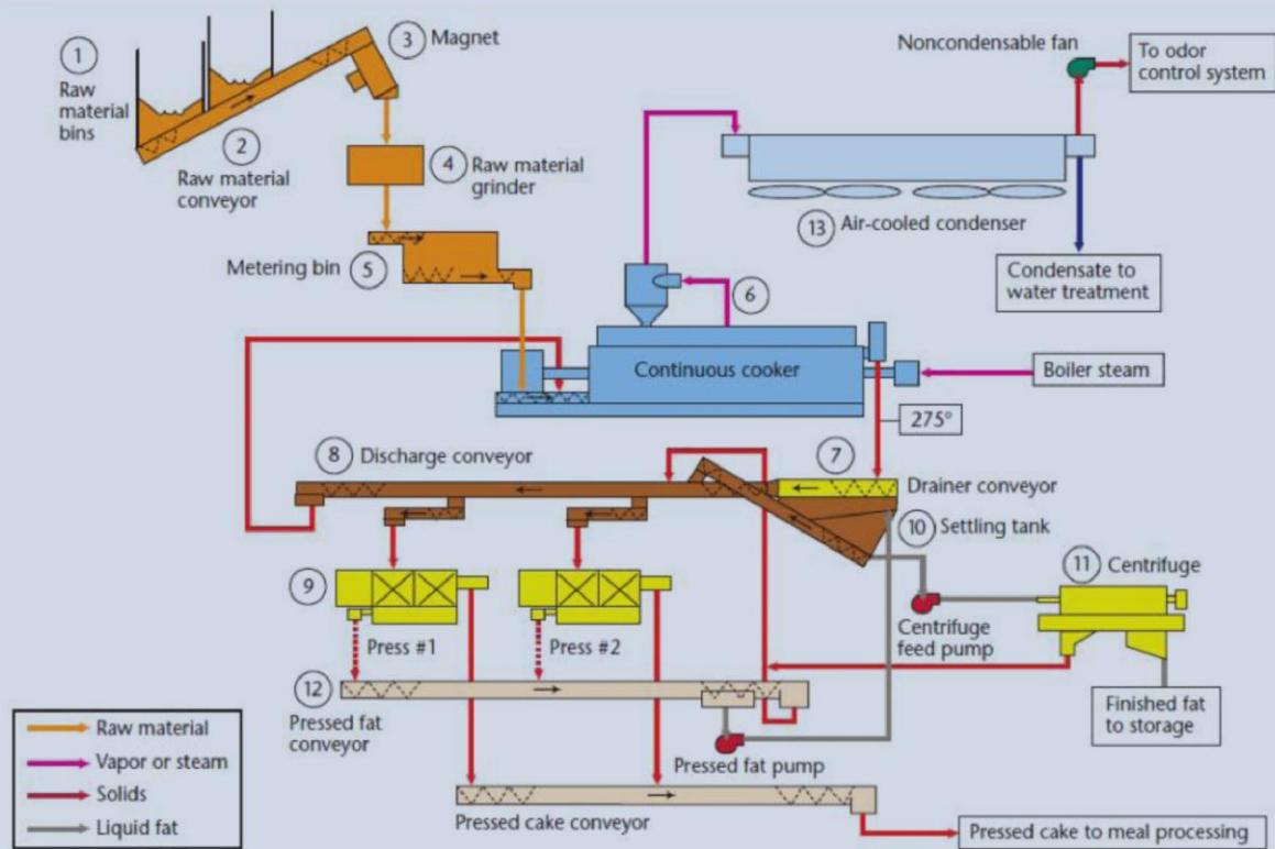
Figure 3. Dry Rendering - Continuous System
